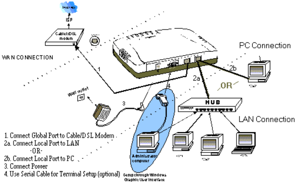
Figure 2: Hardware Connections
