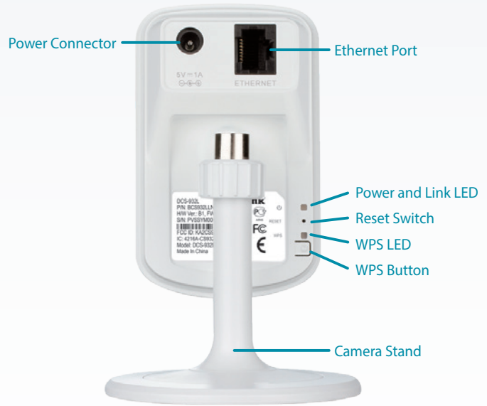
Back View
