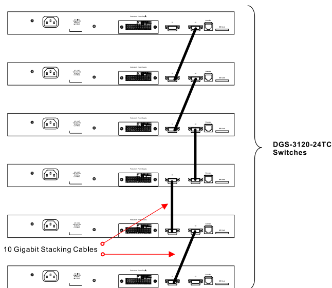
Figure 2-34 Switches stacked in a Duplex Chain
