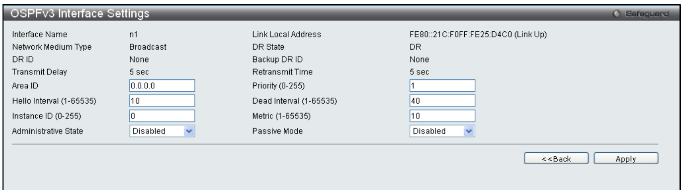
Figure 5-60 OSPFv3 Interface Settings - Edit window
