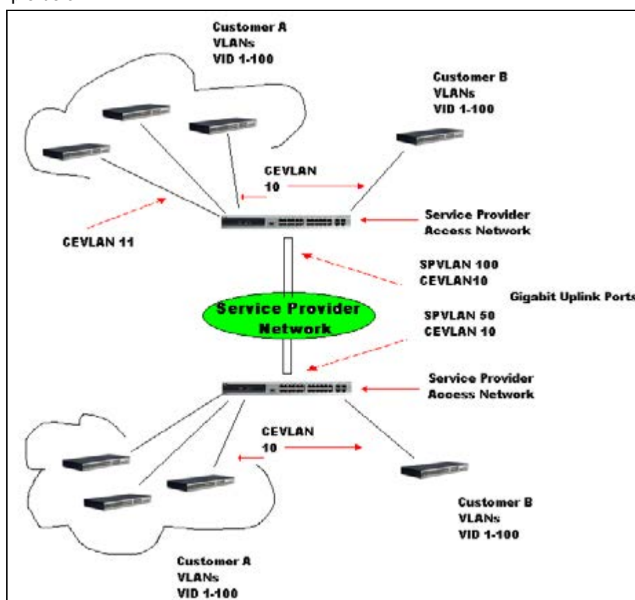
Figure 4-30 QinQ example window
