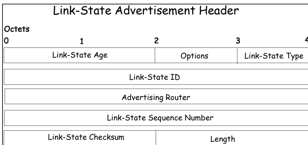
Figure 5-35 Link State Advertisement Header
