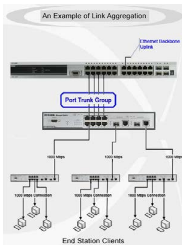
4-39 Example of Port Trunk Group
