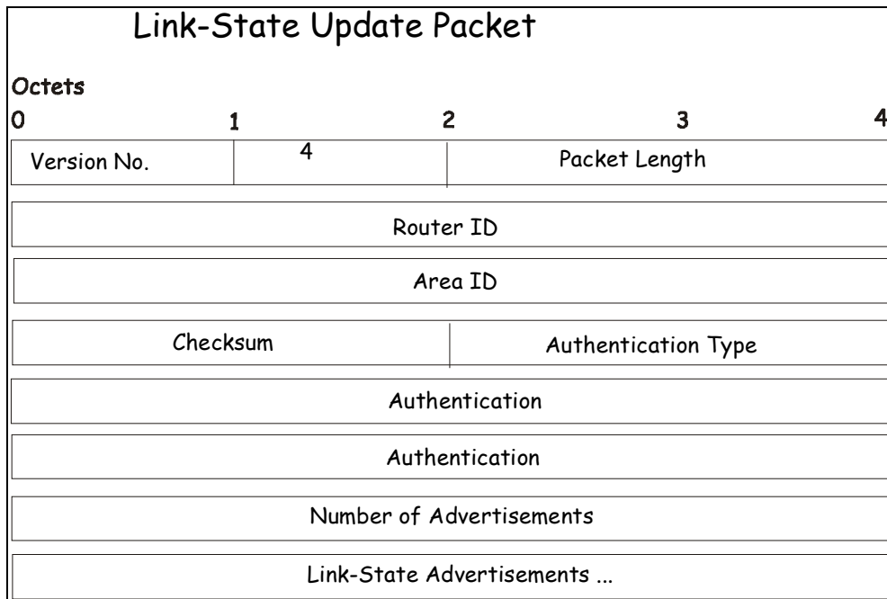
Figure 5-33 Link-State Update Packet
