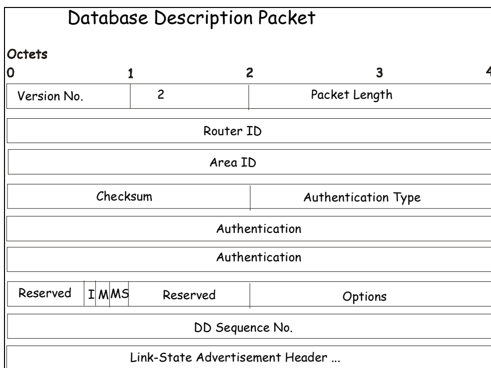
Figure 5-31 Database Description Packet
