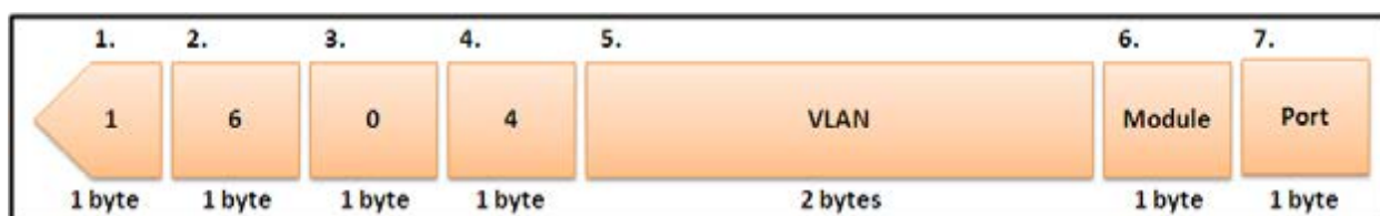
Figure 9-2 Circuit ID Sub-option Format
