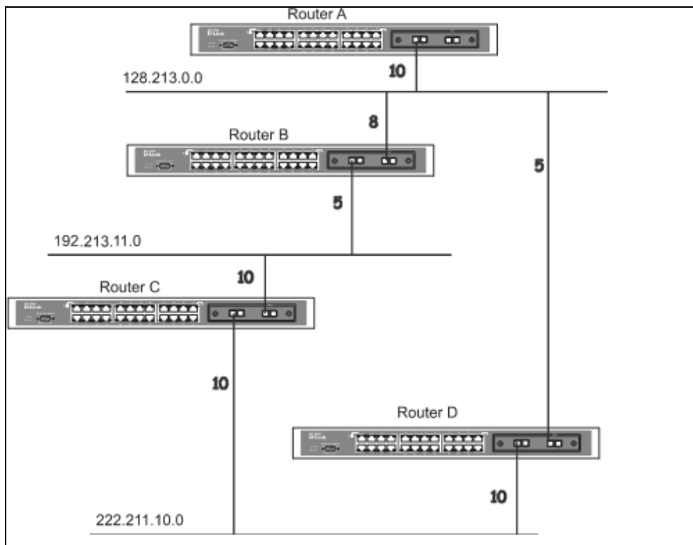
Figure 5-26 Constructing a Shortest Path Tree
