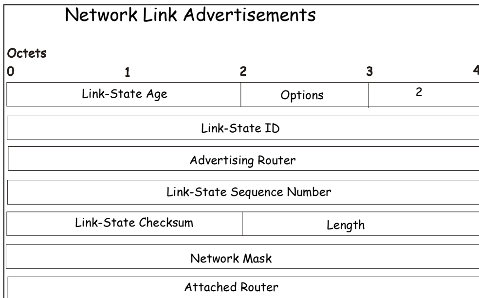
Figure 5-37 Network Link Advertisements
