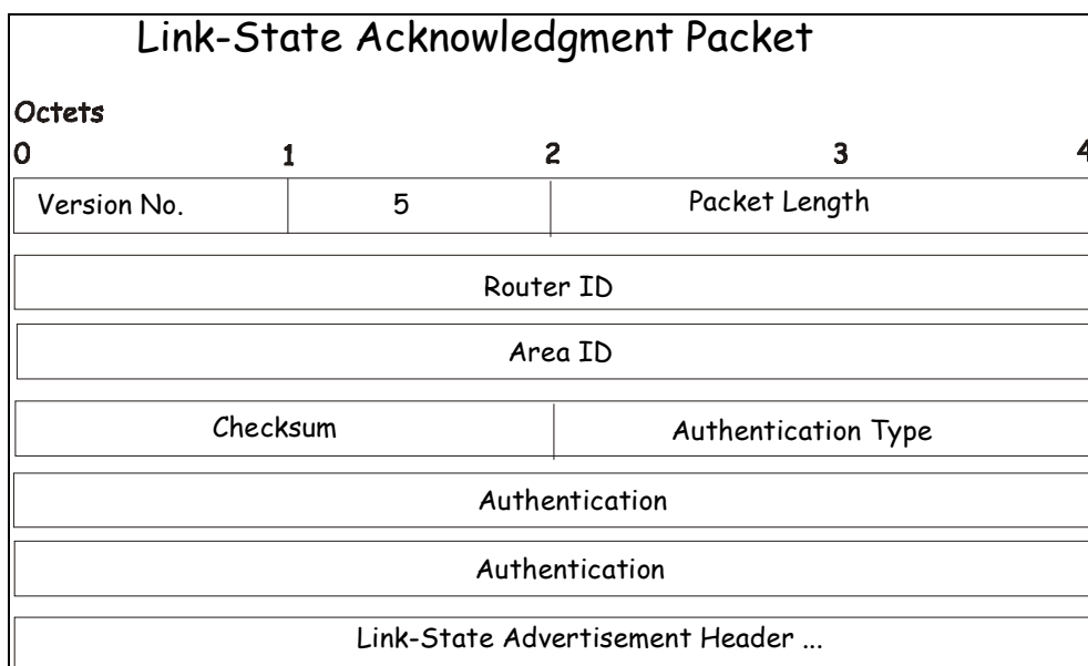
Figure 5-34 Link State Acknowledge Packet
