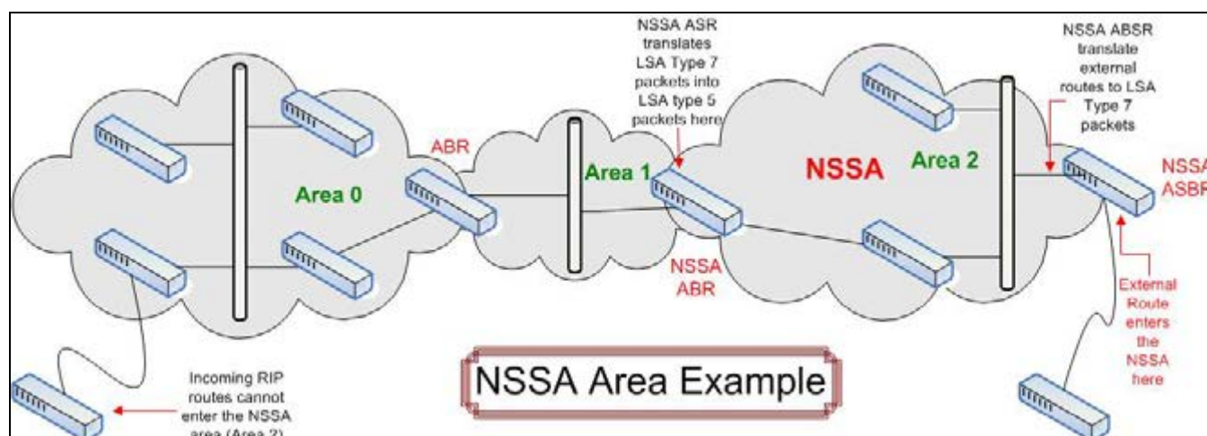
Figure 5-40 NSSA Area example
