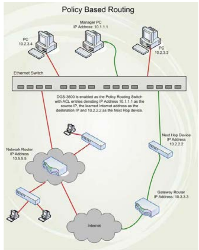
Figure 5-11 Policy Base Routing Example window
