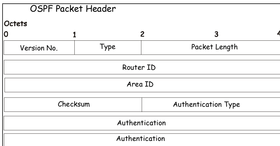
Figure 5-29 OSPF Packet Header Format
