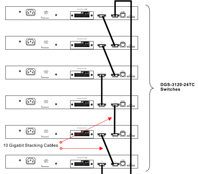
Figure 2-35 Switches stacked in a Duplex Ring
