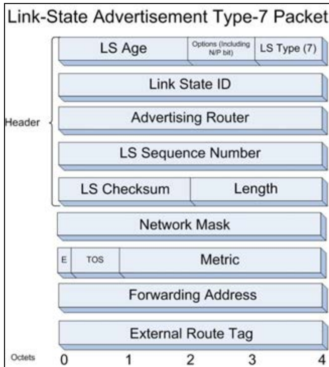
Figure 5-41 LSA Type-7 Packet
