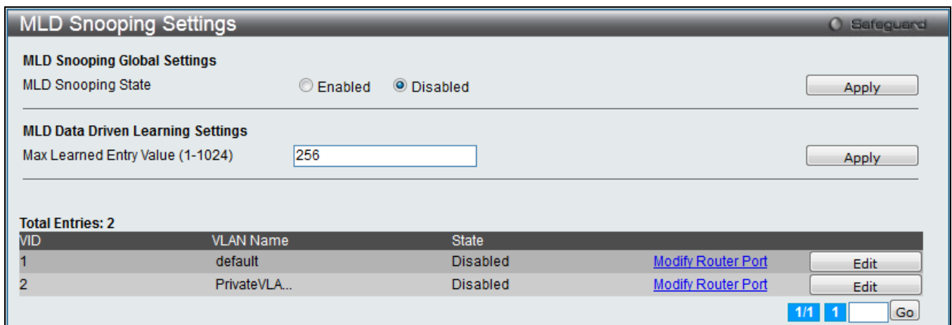
Figure 4-74 MLD Snooping Settings window (EI and SI Mode Only)
