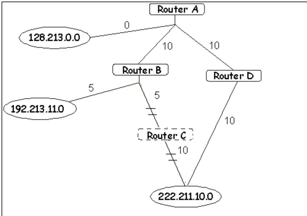
Figure 5-27 Constructing a Shortest Path Tree
