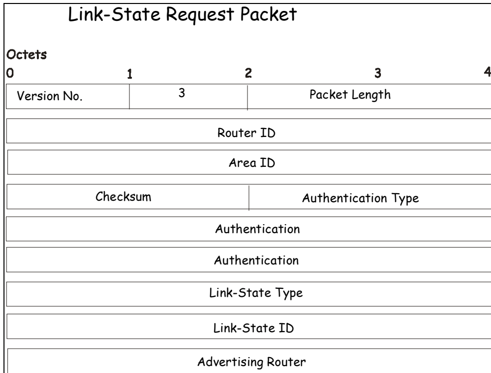
Figure 5-32 Link-State Request Packet
