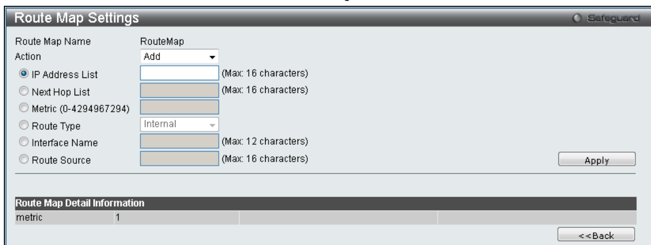
Figure 5-147 Route Map Settings - Match Clause window
