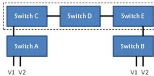
Figure 4-26 Example of VLAN Trunk
