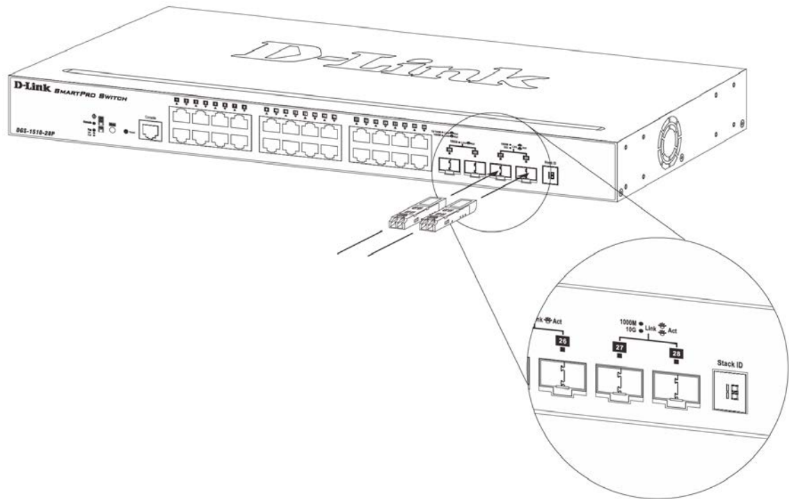
Figure 2–4 Inserting fiber-optic transceivers into a Switch
