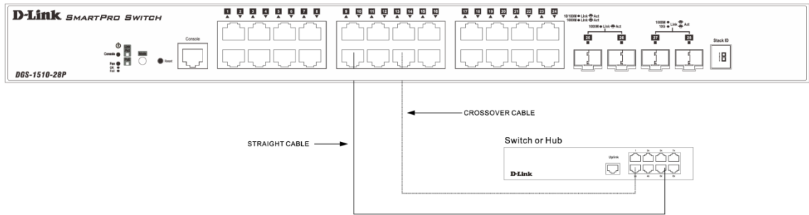
Figure 3–2 Switch to Switch Connection
