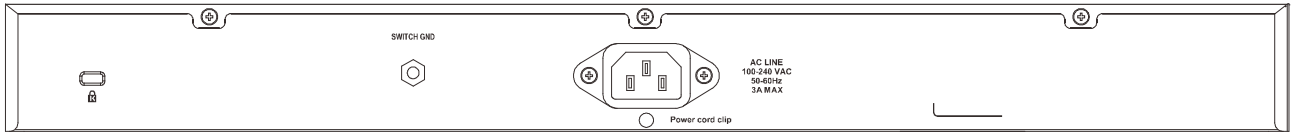
Figure 1-11 Rear panel view of a DGS-1510-28P Switch
