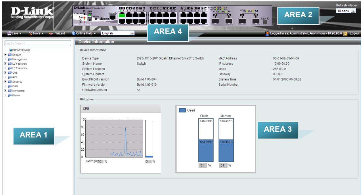
Figure 5-2 Main Web-manager Window
