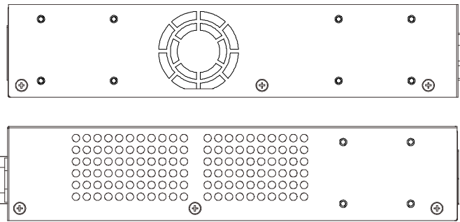
Figure 1–14 Side panels view of a DGS-1510-28 Switch
