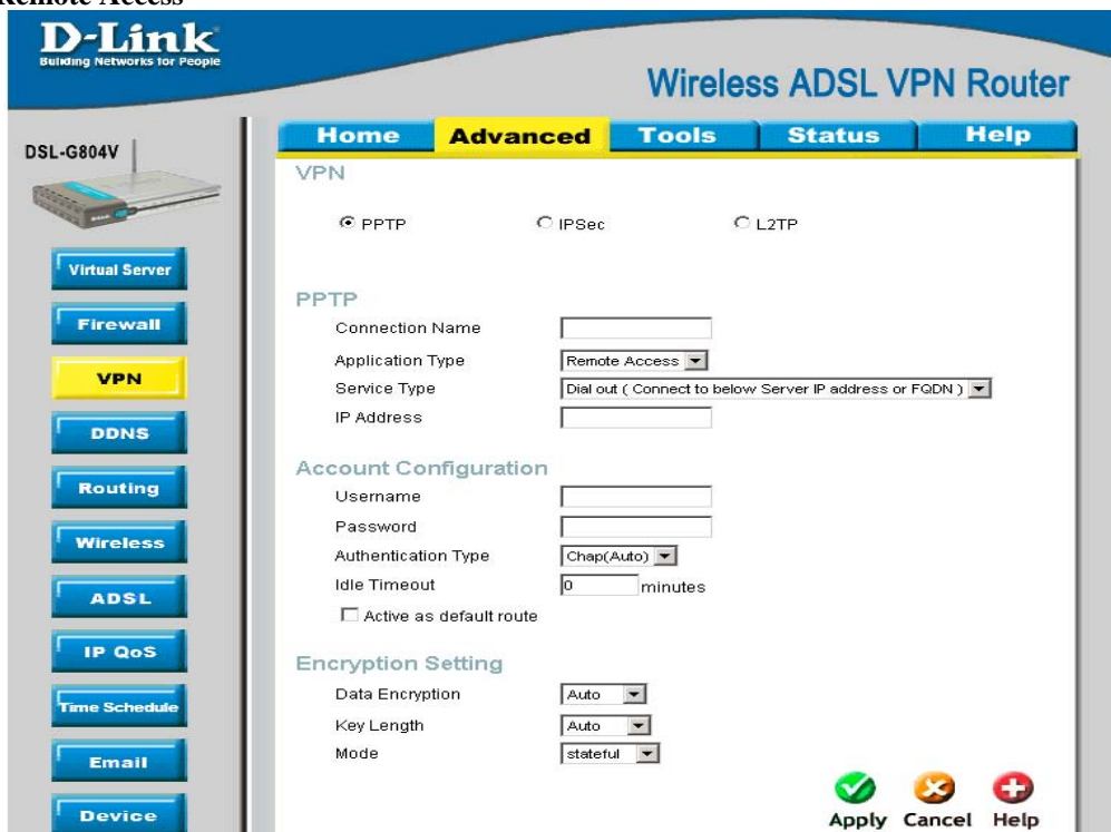
Figure 4-11. VPN – PPTP Remote Access
