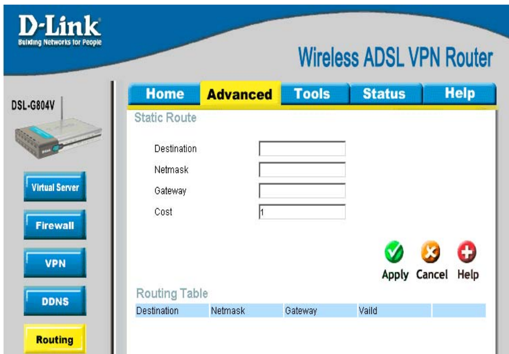
Figure 4-19. Routing (Static Route)
