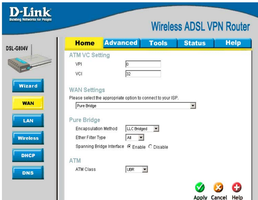
Figure 3-8. WAN Setup window – Pure Bridge
