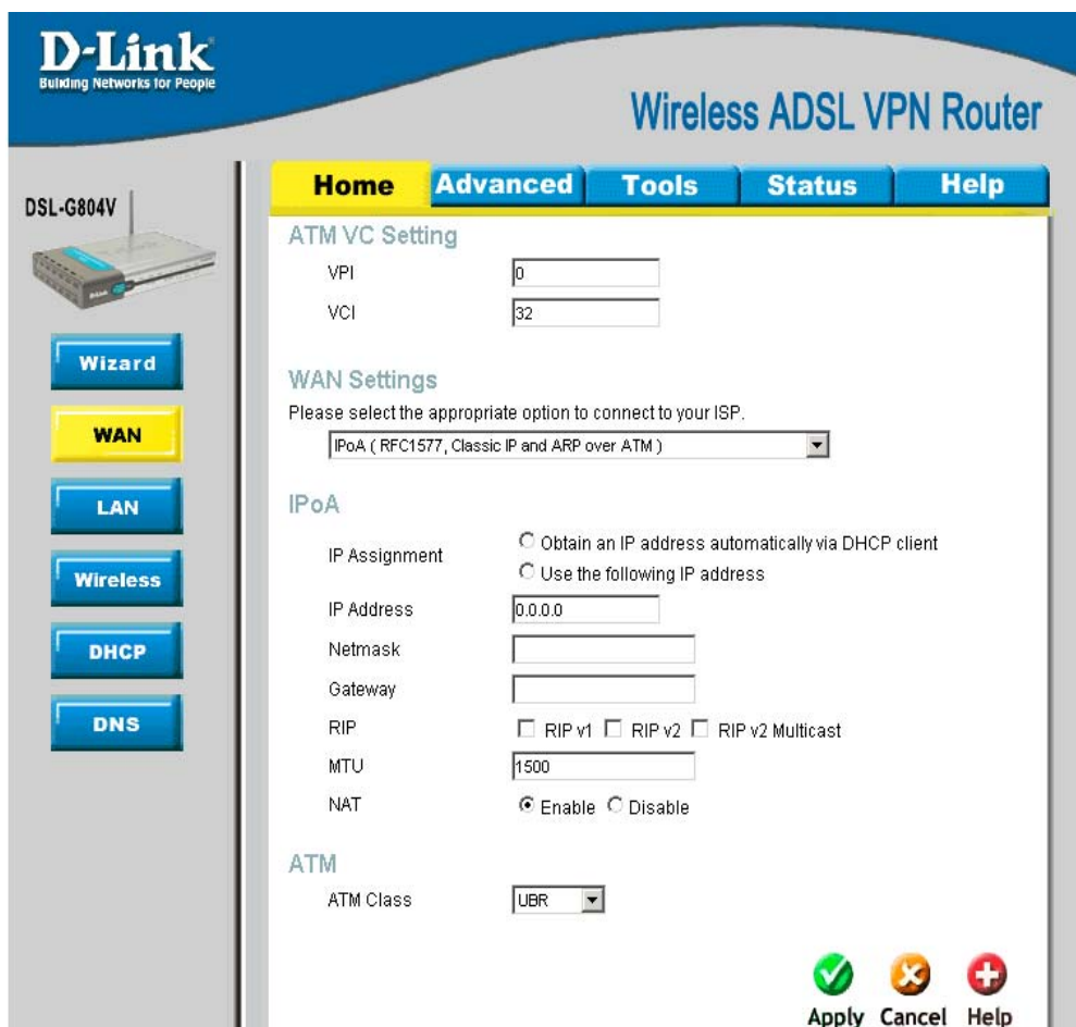
Figure 3-7. WAN Setup window - IPoA
