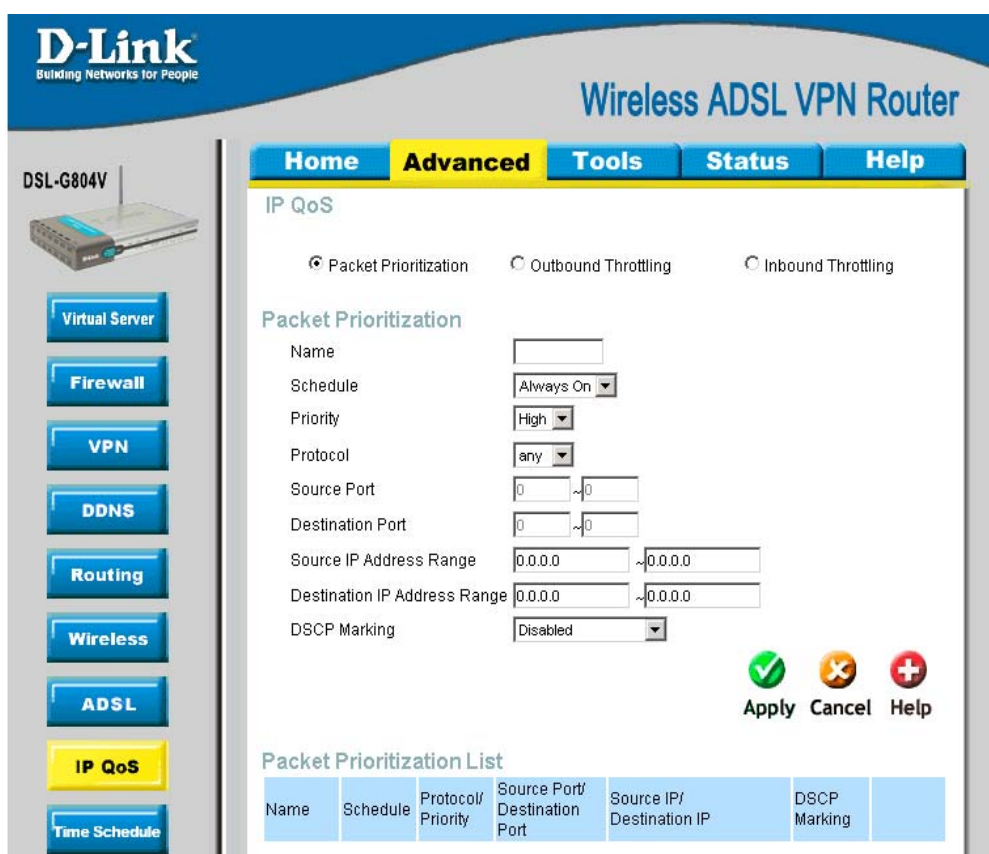
Figure 4-24. IP QoS – Packet Prioritization
