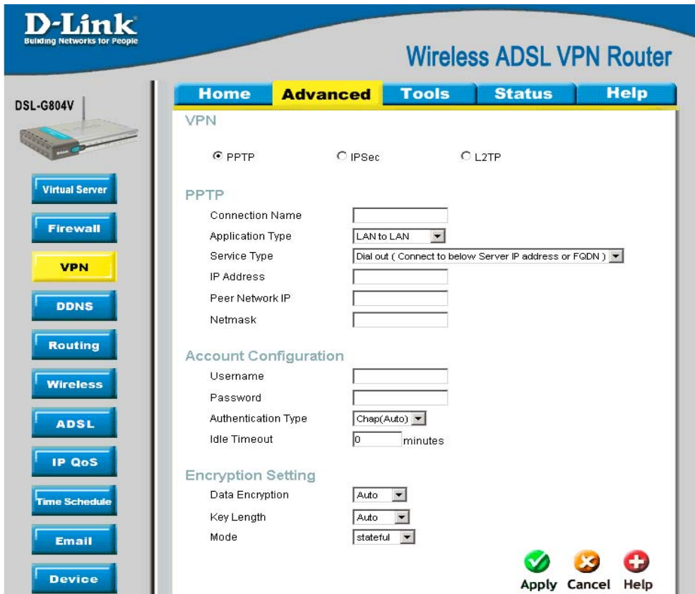
Figure 4-12. VPN – PPTP LAN to LAN
