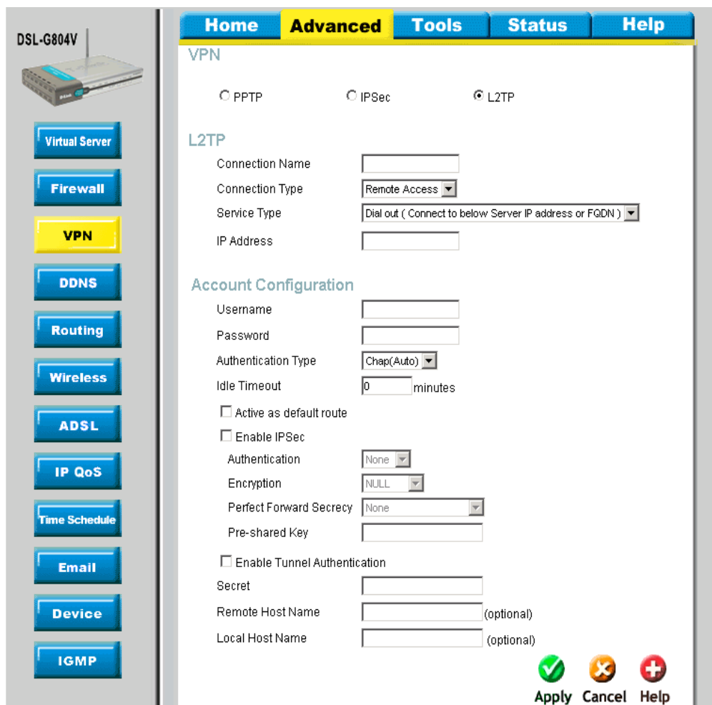
Figure 4-16. VPN – L2TP Remote Access
