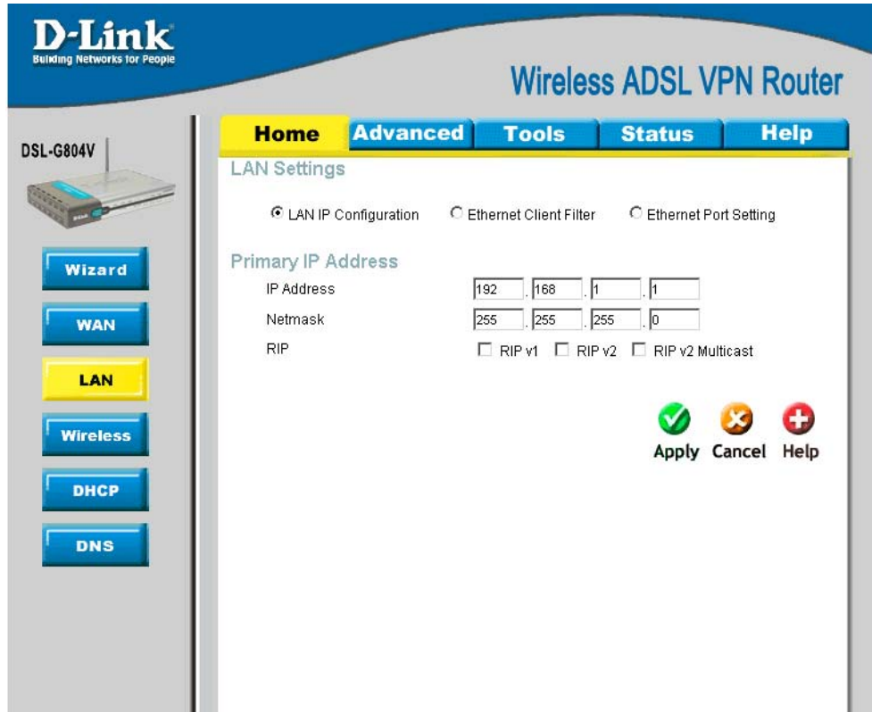
Figure 3-9. Home – LAN Settings (LAN IP Configuration)
