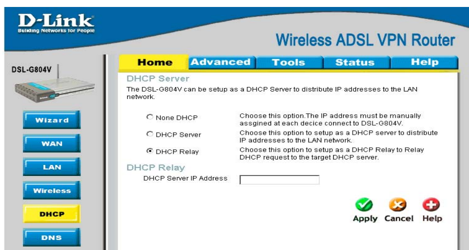
Figure 3-15. Home – DHCP Server (DHCP Relay)
