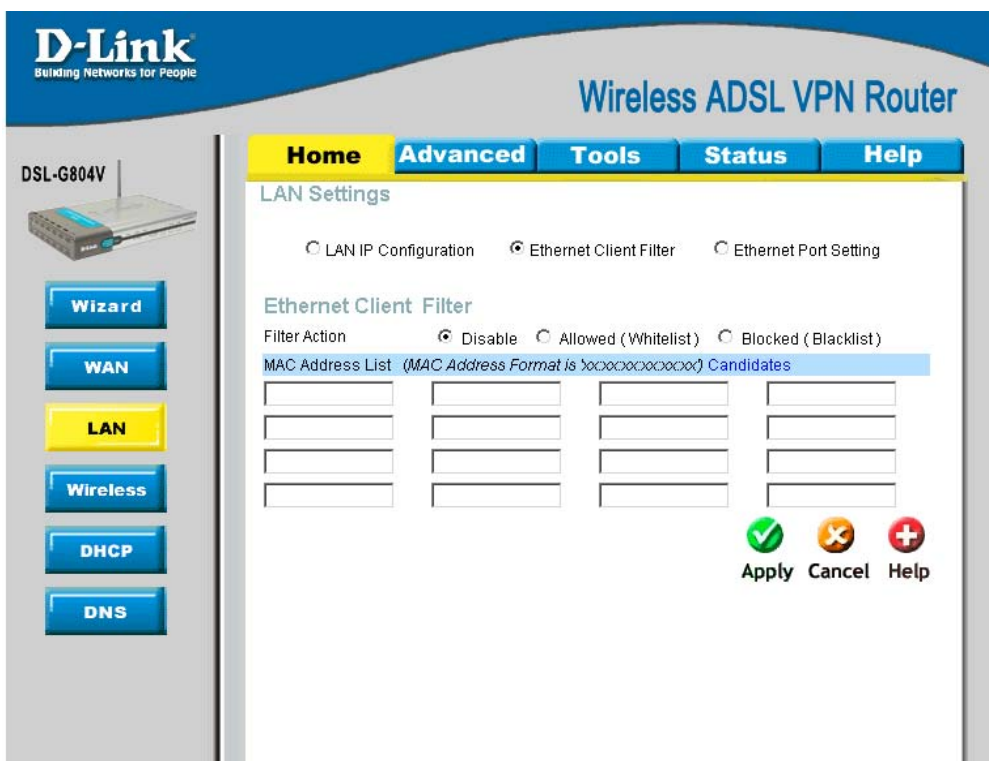
Figure 3-10. Home – LAN Settings (Ethernet Client Filter)
