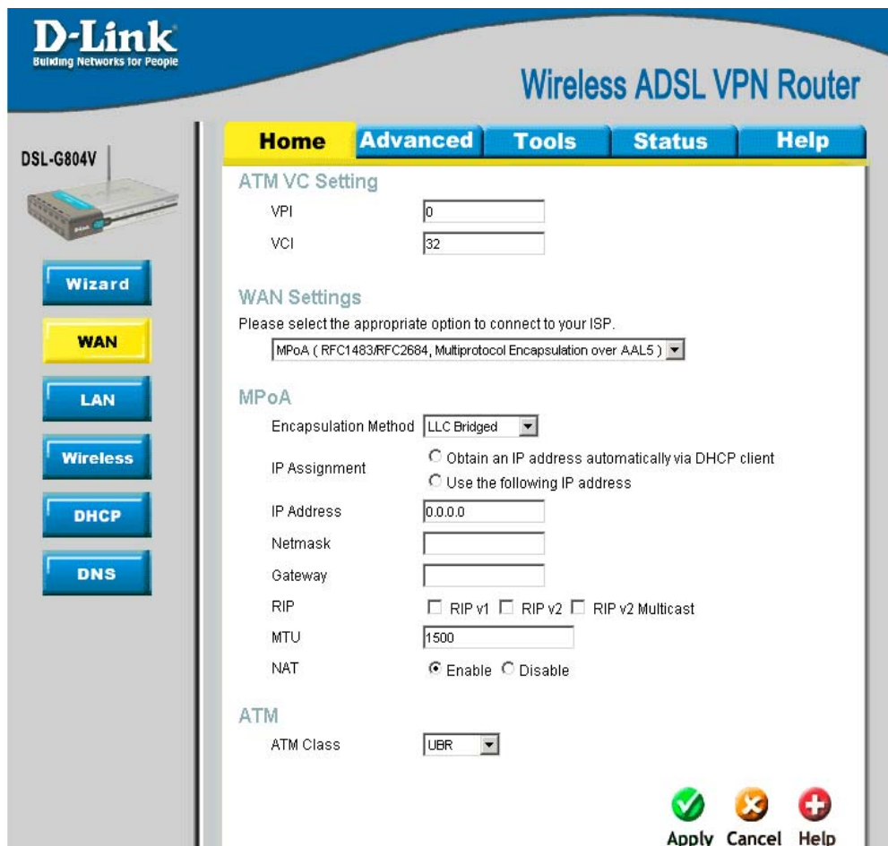
Figure 3-6. WAN Setup window - MPoA
