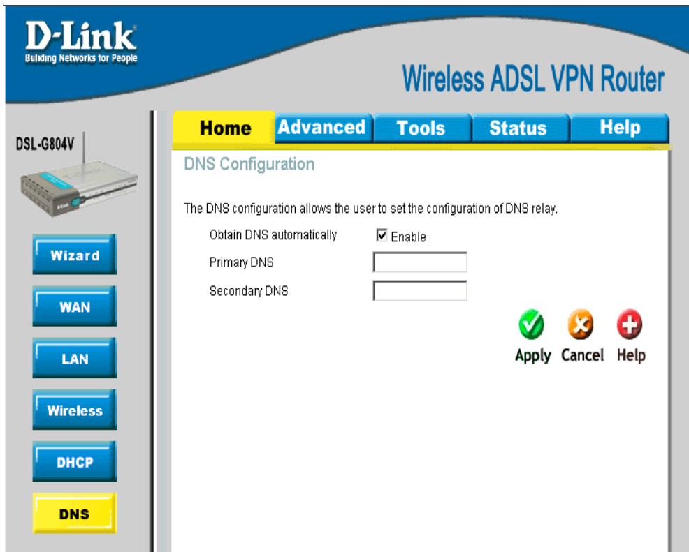
Figure 3-16. Home – DNS Configuration
