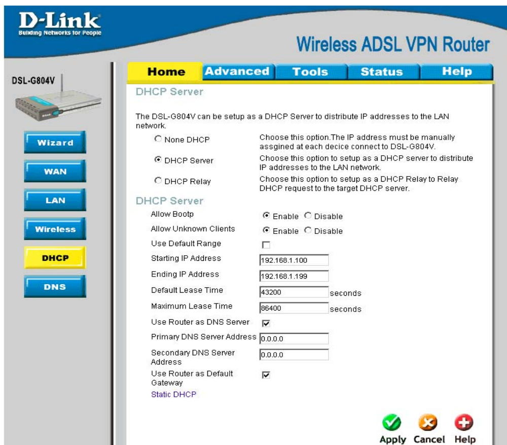
Figure 3-13. Home – DHCP Server
