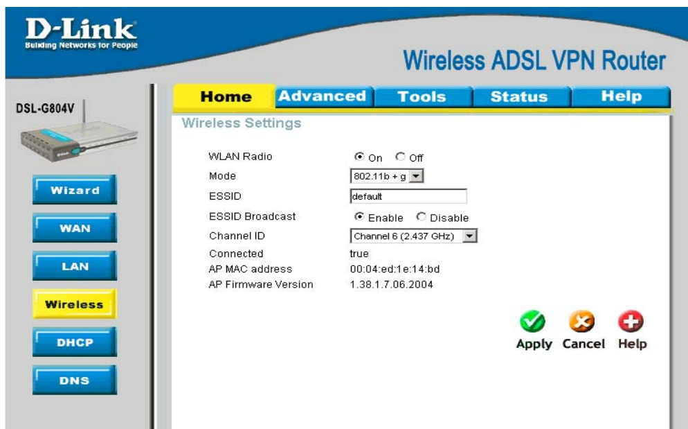
Figure 3-12. Home – Wireless Settings
