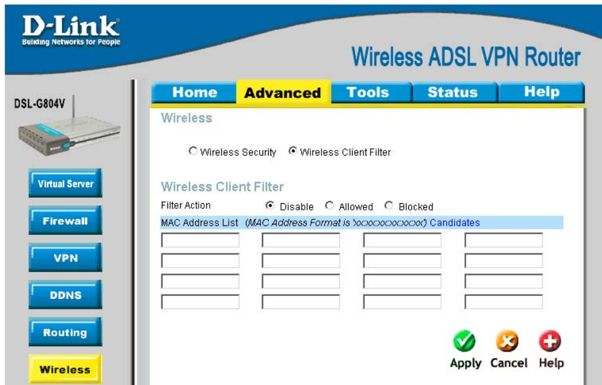
Figure 4-20. Wireless Client (MAC) Filter
