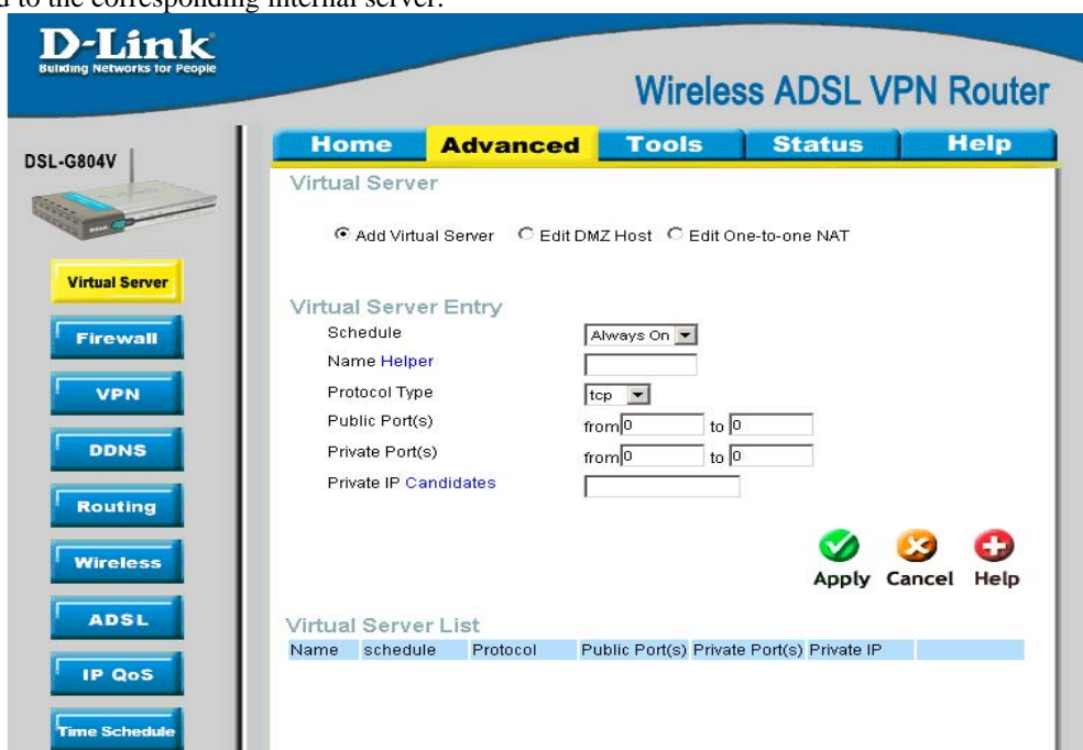
Figure 4-1. Virtual Server – Add Virtual Server
