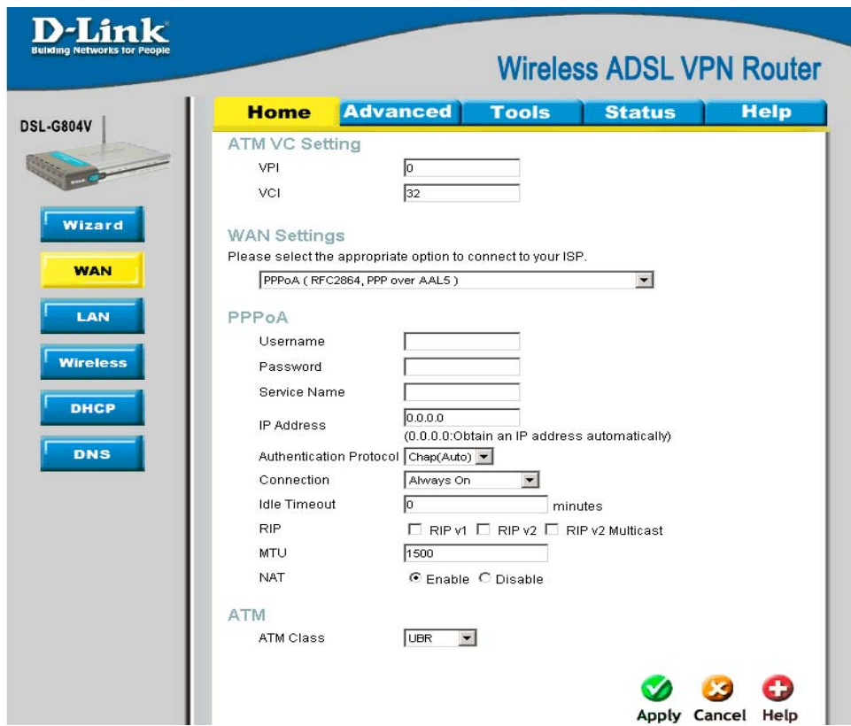
Figure 3-5. WAN Setup window - PPPoA
