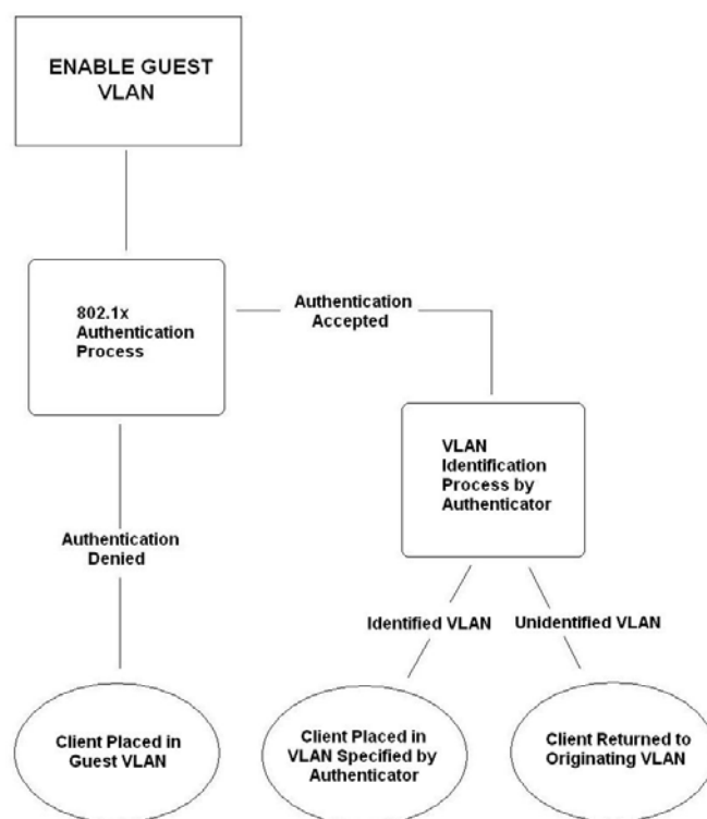
Figure 6- 101 Guest VLAN Authentication Process
