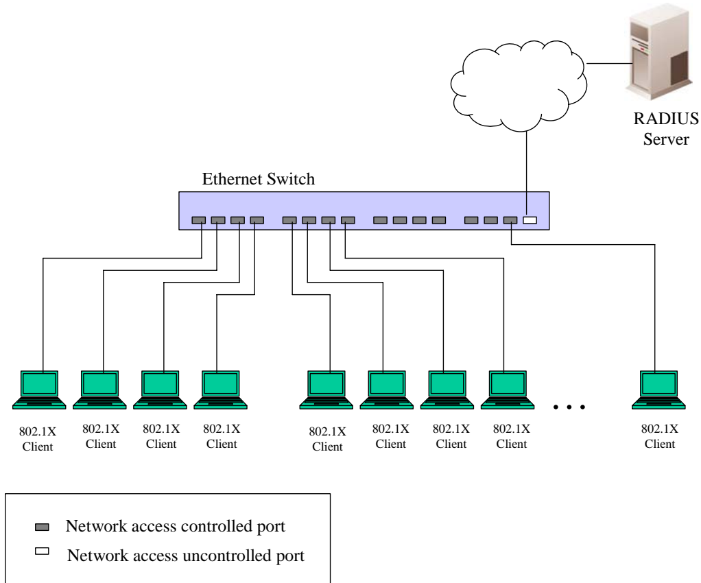
Figure 6- 92. Example of Typical Port-Based Configuration
