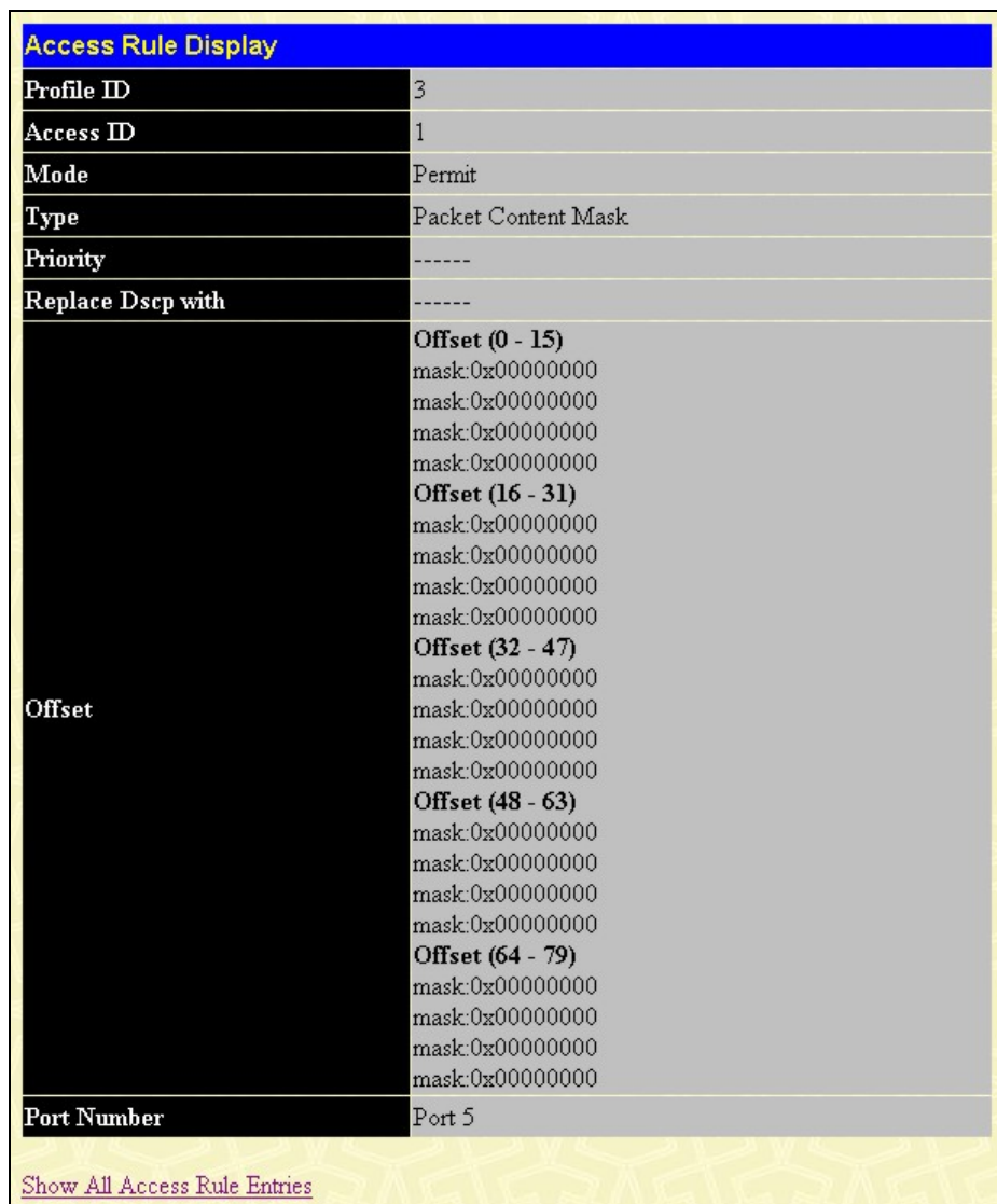
Figure 6- 74. Access Rule Display window (Packet Content)
