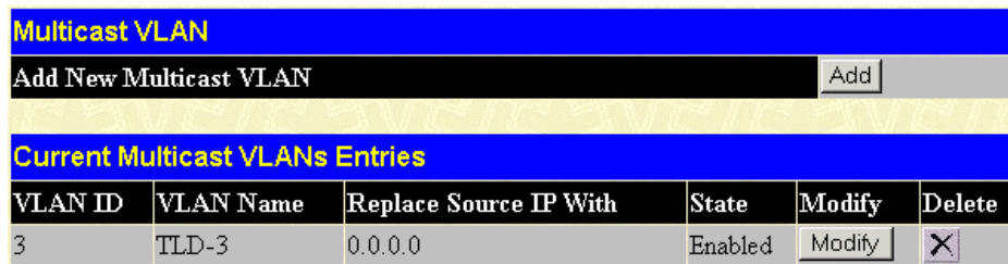
Figure 6- 20 Multicast VLAN and Current Multicast VLANs Entries Table
