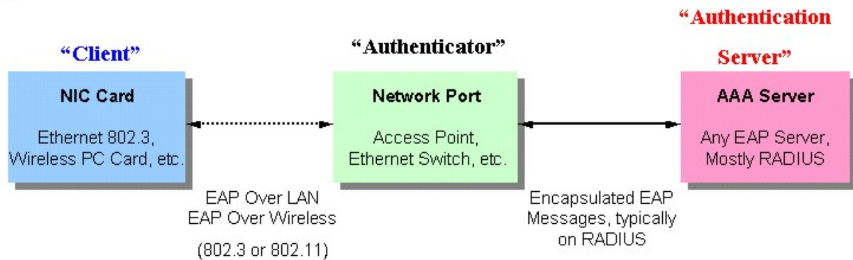
Figure 6- 88. Three Functions of 802.1x
