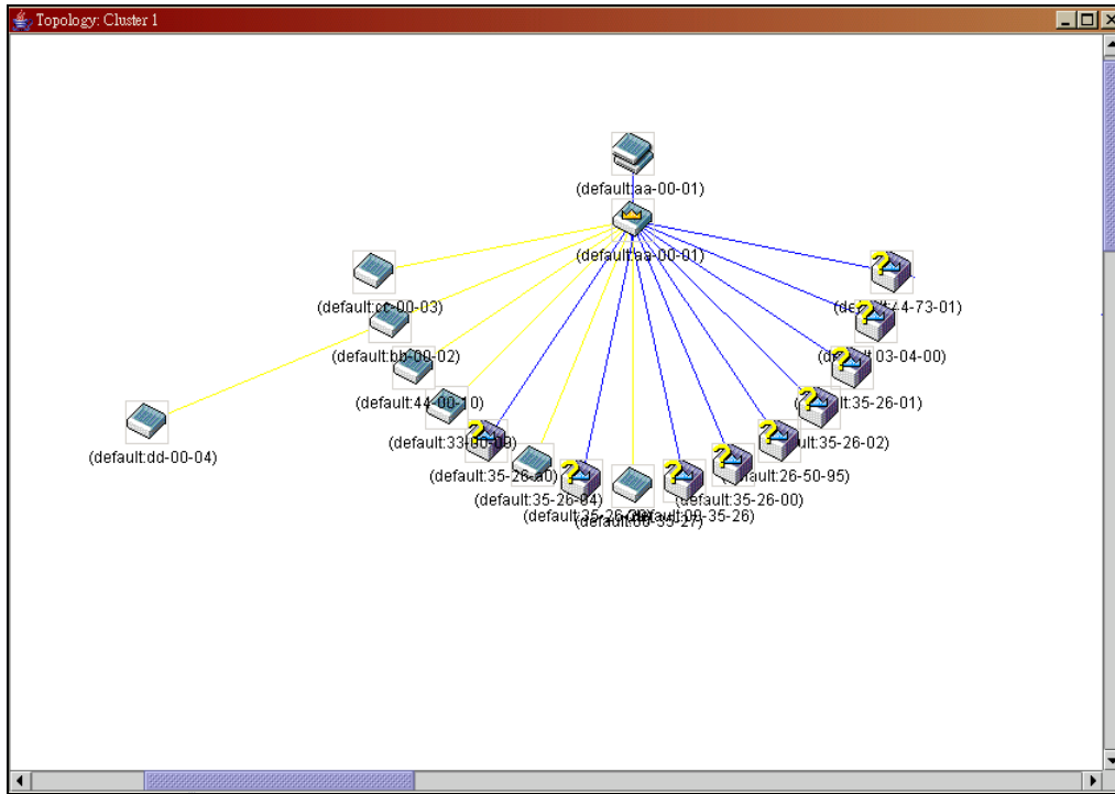
Figure 10- 5. Topology view
