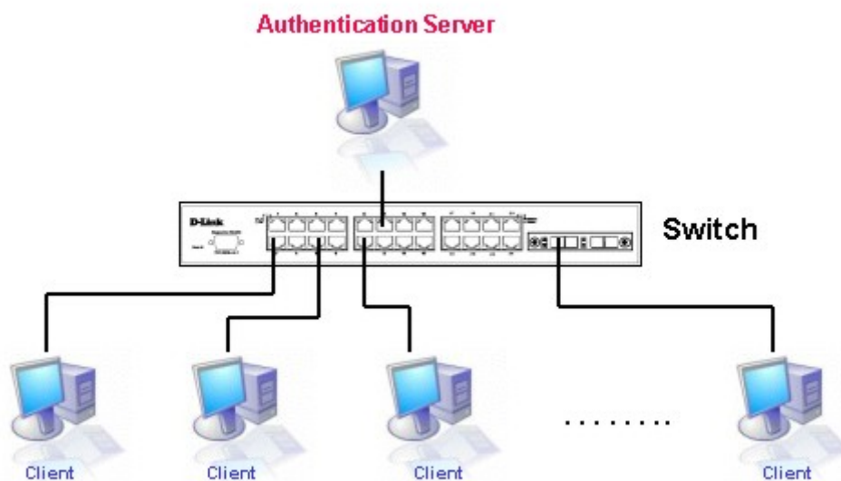
Figure 6- 89. Authentication Server
