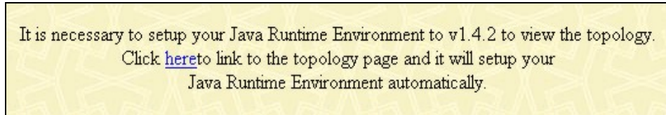
Figure 10- 3. Java window
