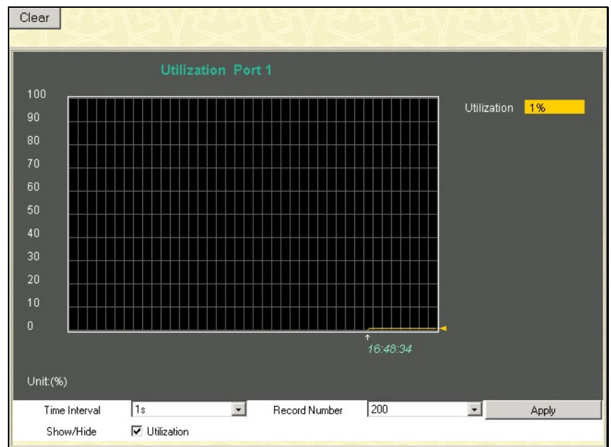
Figure 8- 1. Utilization window
