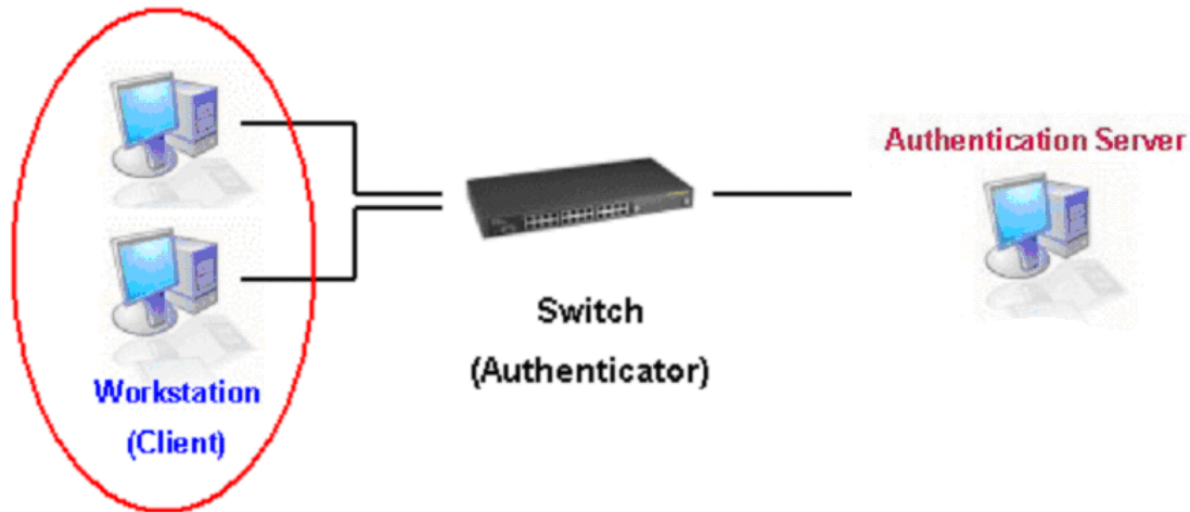
Figure 6- 91. Client
