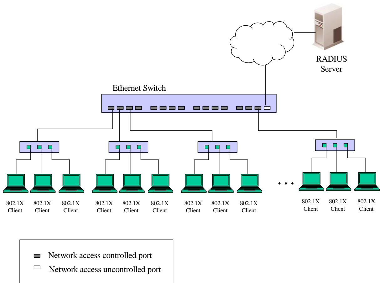
Figure 6- 93. Example of Typical MAC-Based Configuration
