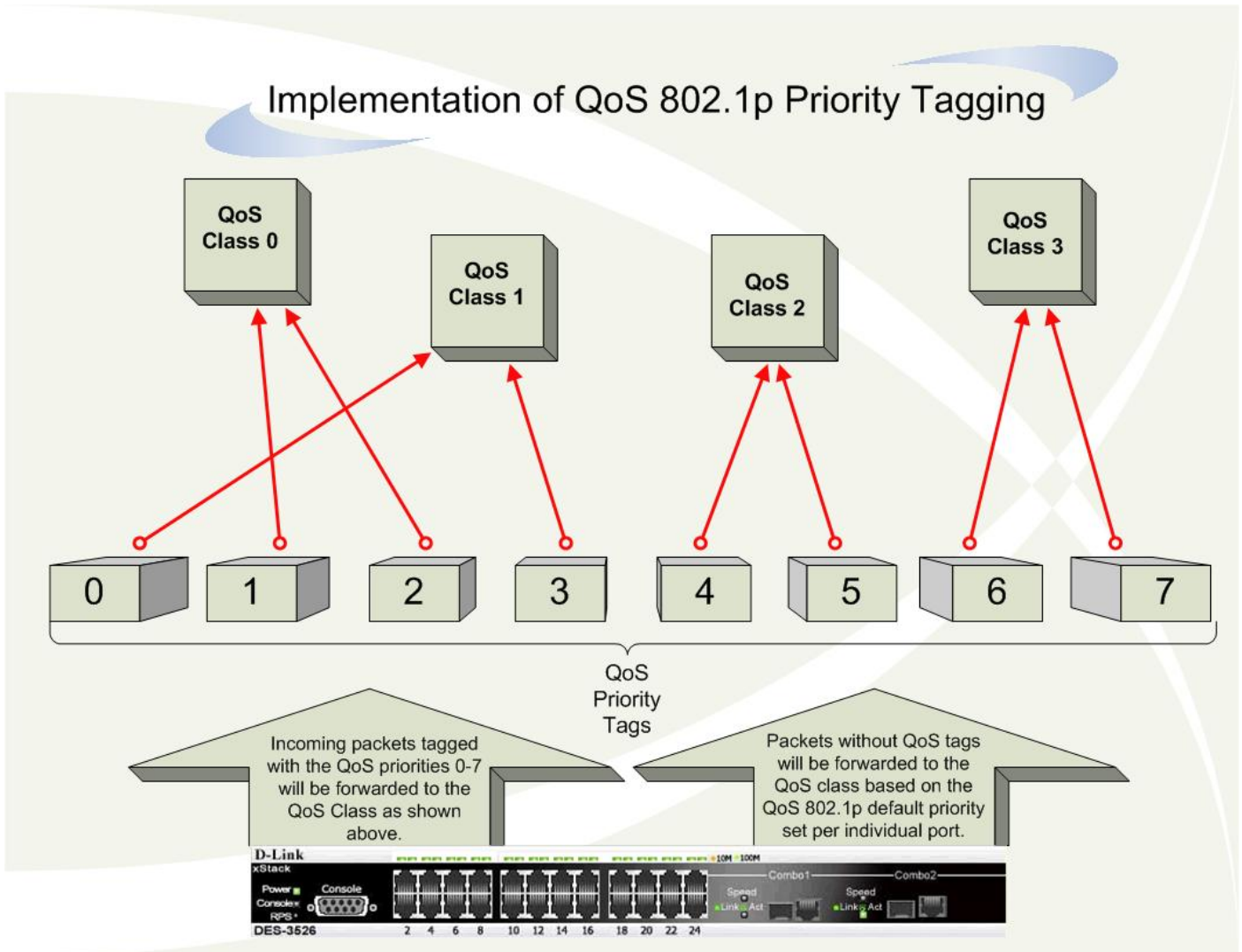
Figure 6- 50. Mapping QoS on the Switch
