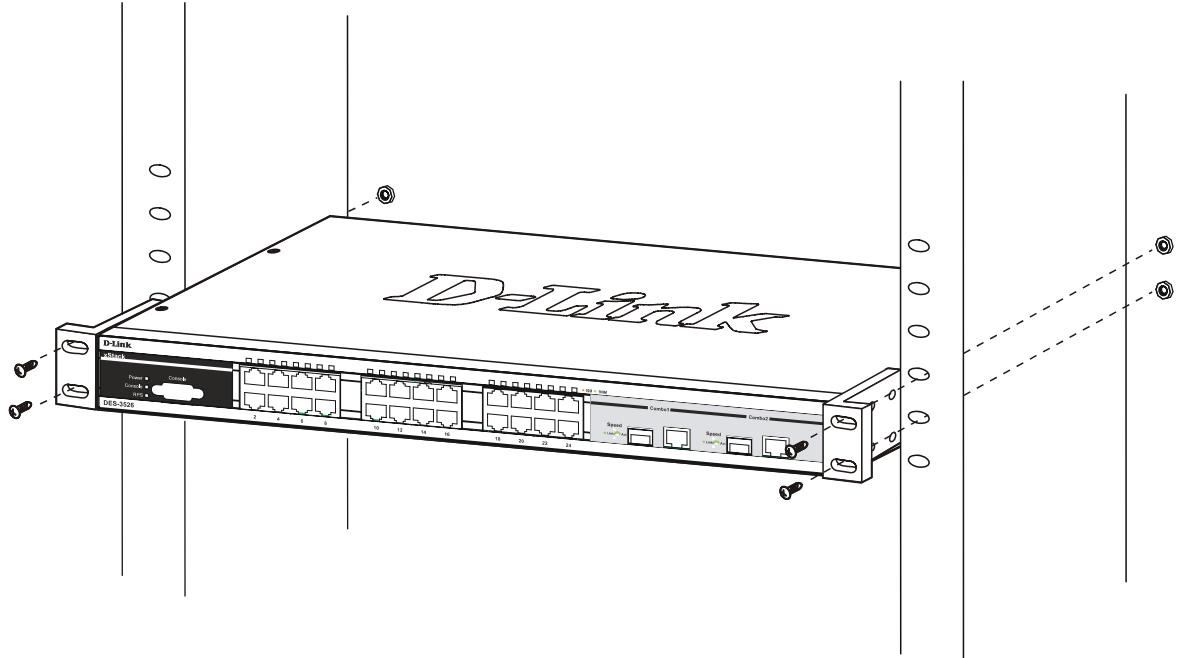
Figure 2- 3. Installing the DES-3526 in a rack
