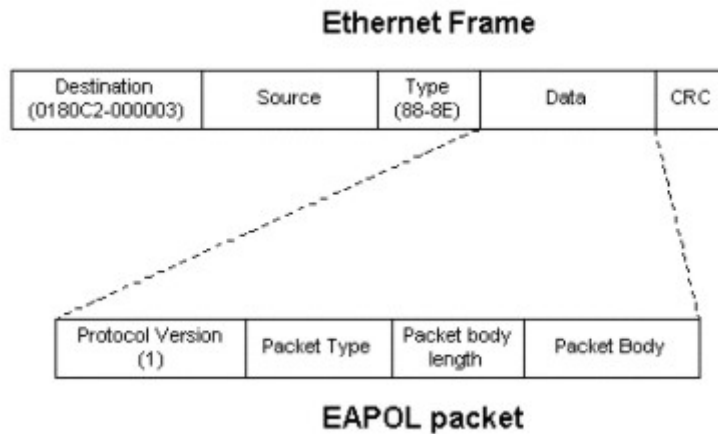
Figure 6- 87. EAPOL Packet
