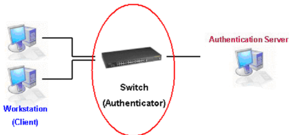
Figure 6- 90. Authenticator
