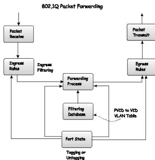
Figure 6- 35. IEEE 802.1Q Packet Forwarding
