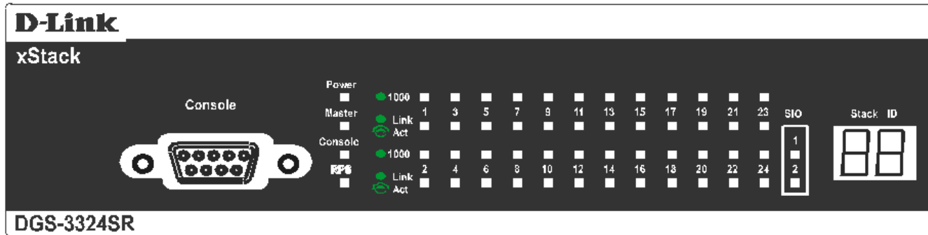
Figure 1- 6. LED Indicators
