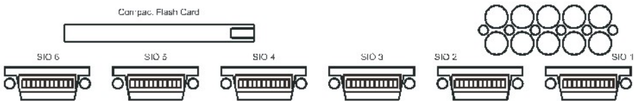
Figure 3- 6. SIO 1-6 Stacking ports at the rear of the DGS-3324SRi
