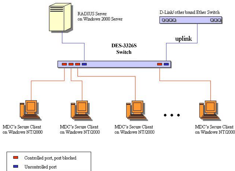
Figure 14- 14. Typical 802.1X Configuration Prior to User Authentication
