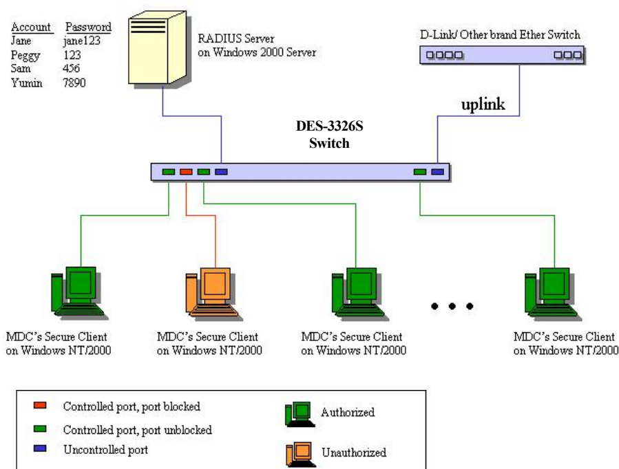
Figure 14- 15. Typical 802.1X Configuration with User Authentication
