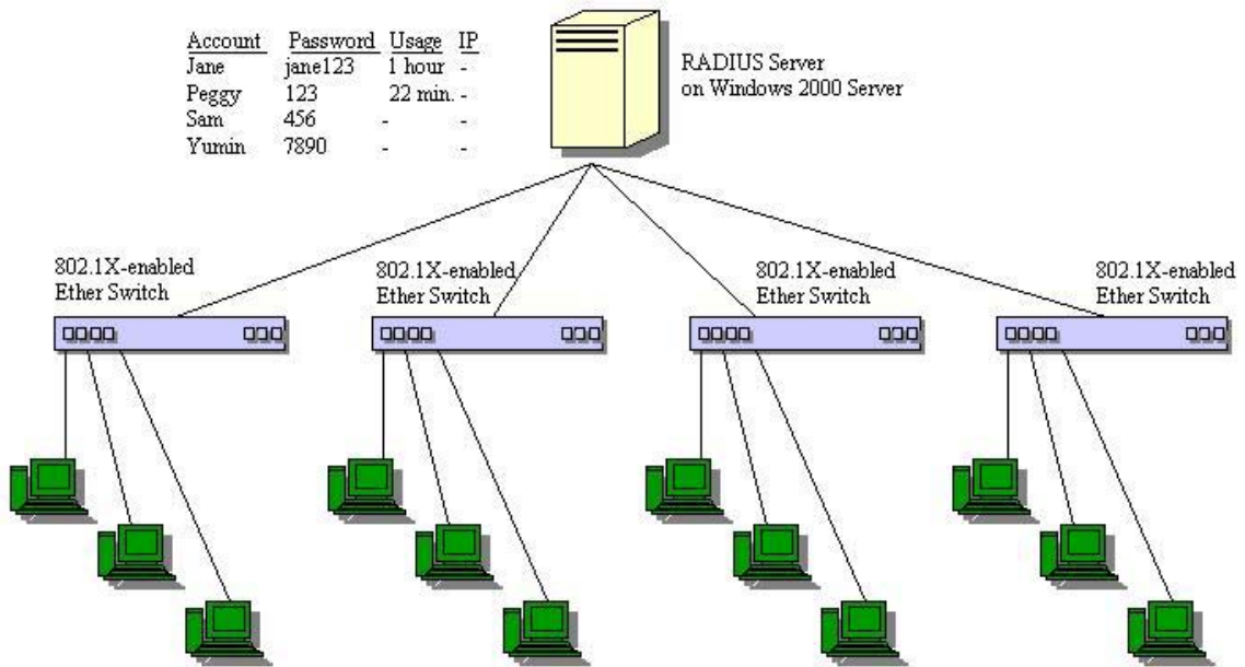
Figure 14- 16. Typical Configuration with 802.1X Fully Implemented
