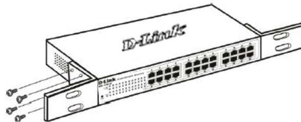
Figure 2. Attaching the mounting brackets
